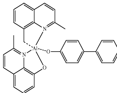
BAIq
