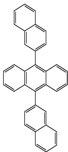
DNA
